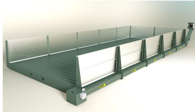
Hydropad wash rack; 16' wide X 37.5' long, drive on back off design. 4' high walls on 3 sides and drag conveyor for automatic solids removal. Example only.....design exactly what you need.
